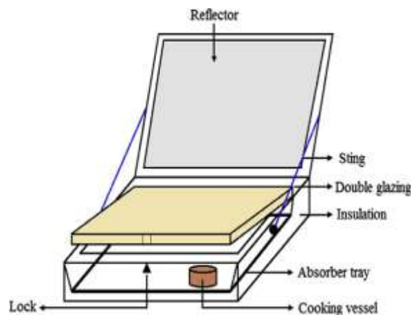
Fig. 2 Box Type Solar Cooker [7]
